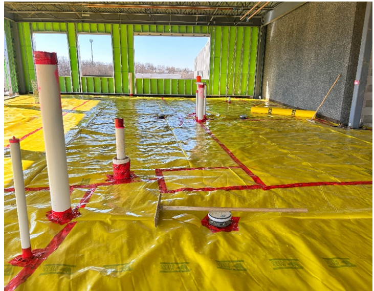
Stego Wrap Vapor Barrier Install Beneath All Slab on Grade Concrete
